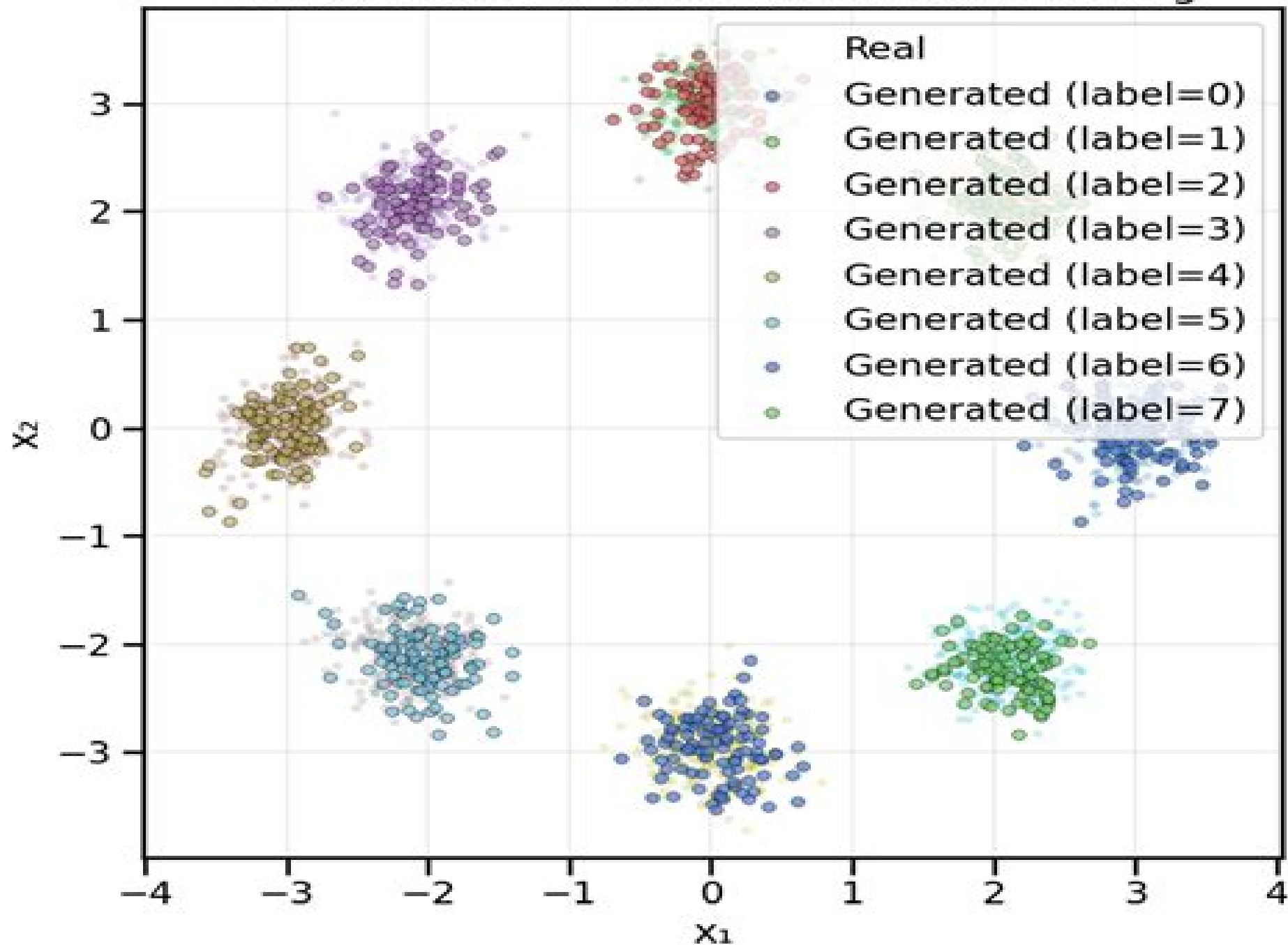
Conditional Flow: One-Hot Mode Conditioning
