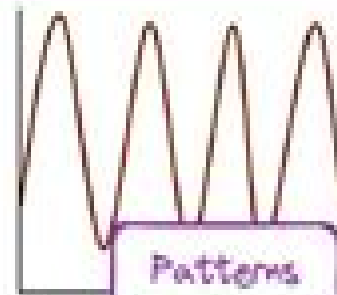
Correlation
