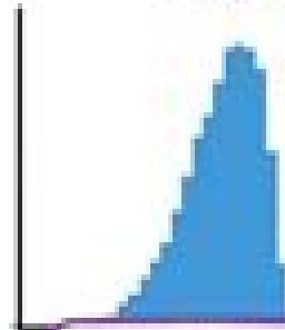
Data distribution
