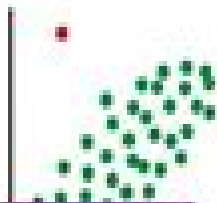
Outliers
