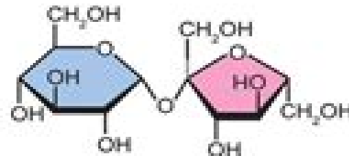
Sucrose
