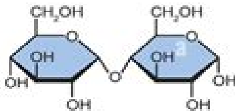
Maltose
