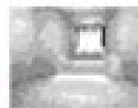
Light Map
