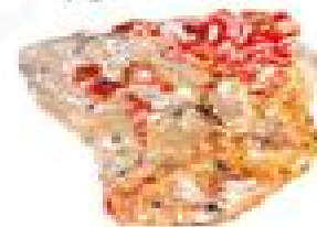
vanadinite
