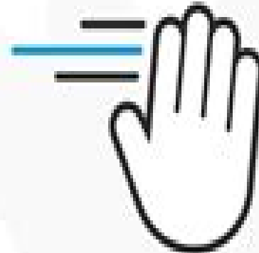
Gesture-based Interfaces
