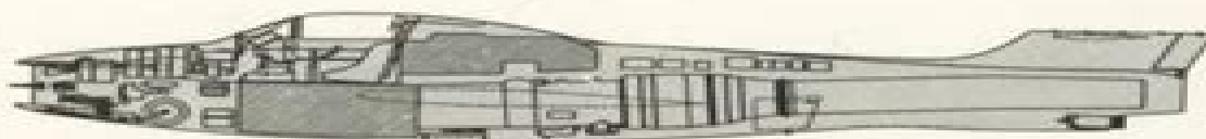
F-84F CUTAWAY (W/LR-63-AJ-1)
