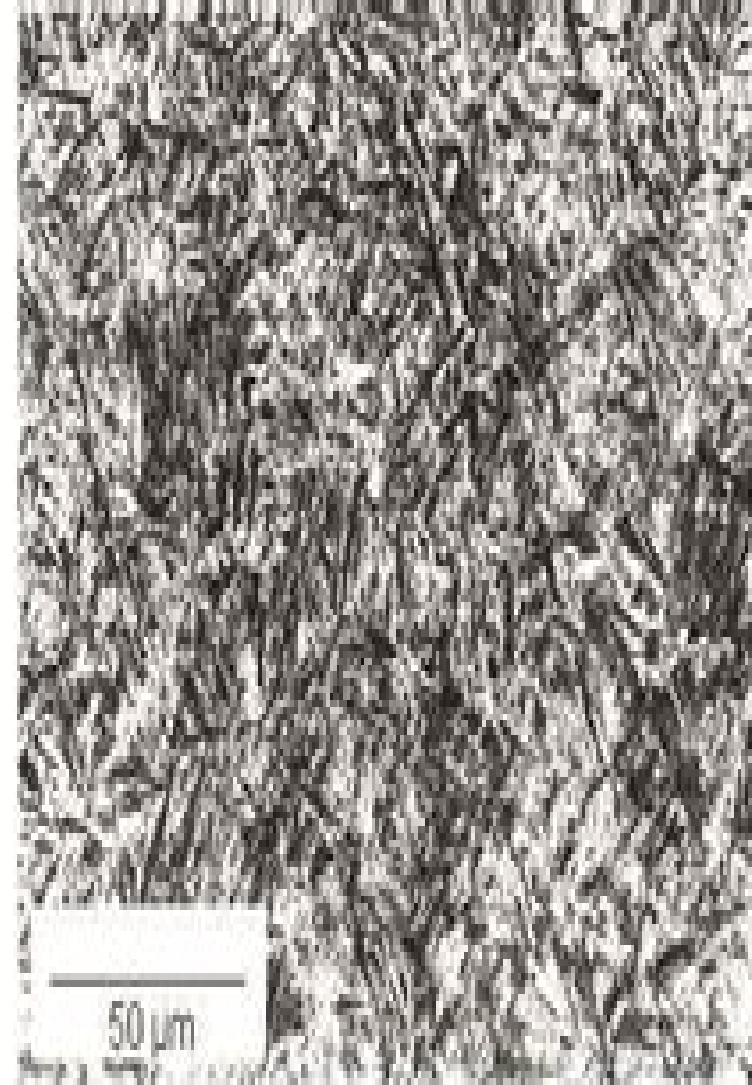
Figure 10 - Typical martensitic microstructure
