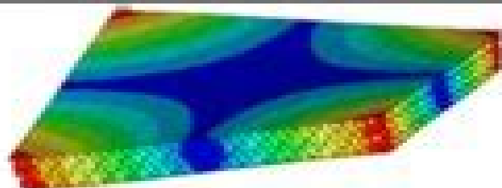
Mode 1: 1868.0 Hz.
