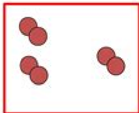
Element
