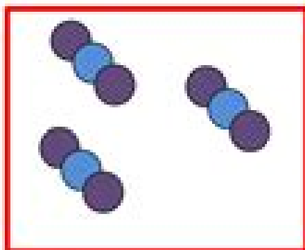
Compound
