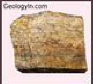
Mylonite
