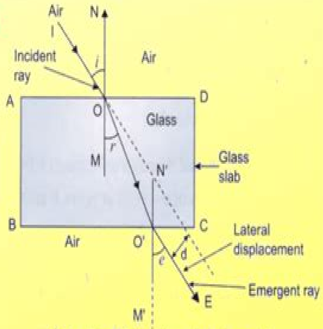
Refraction of light through a glass slab
