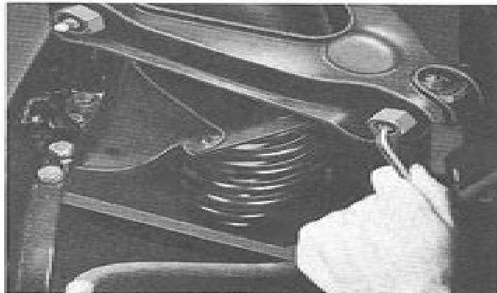
Fig. 1—Turning Pivot Pin to Set Caster and Camber
