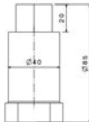
Auxiliary view B Scale: 1:1
