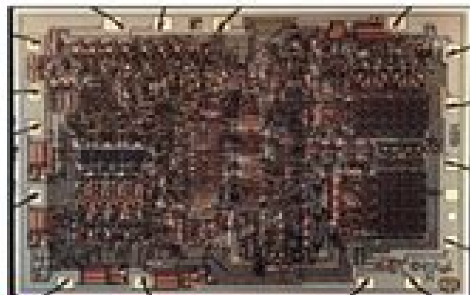
Intel 4004 4-bit \mu Proc 1000 Trs, 1 MHz operation
