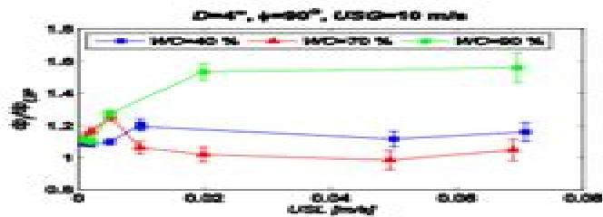
Figure 2: Frictional pressure drop normalized with the two-phase gas-oil pressure drop plotted versus USL.
