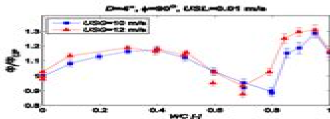
Figure 1: Frictional pressure drop normalized with the two-phase gas-oil pressure drop plotted versus water cut.
