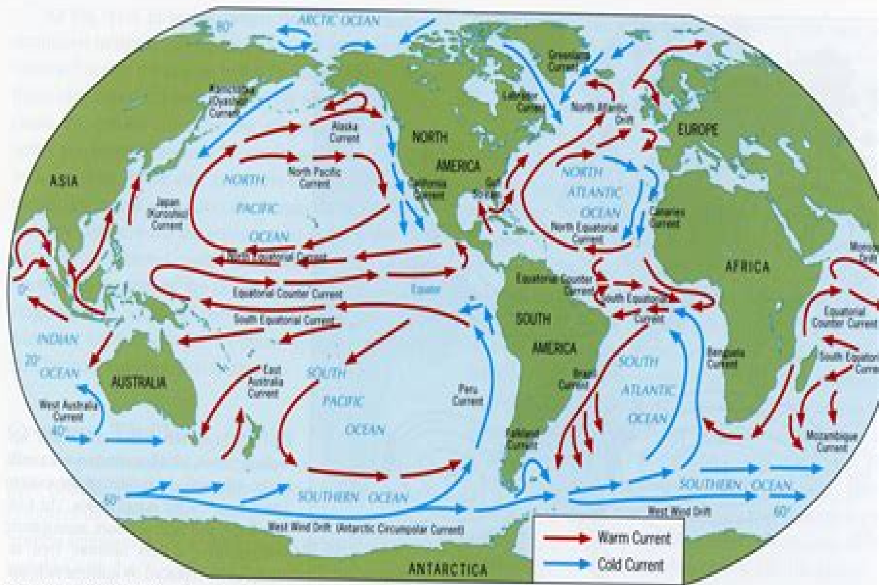
FIGURE 11-6 World distribution of ocean currents, showing average positions and relative temperatures in each of the ocean basins.
