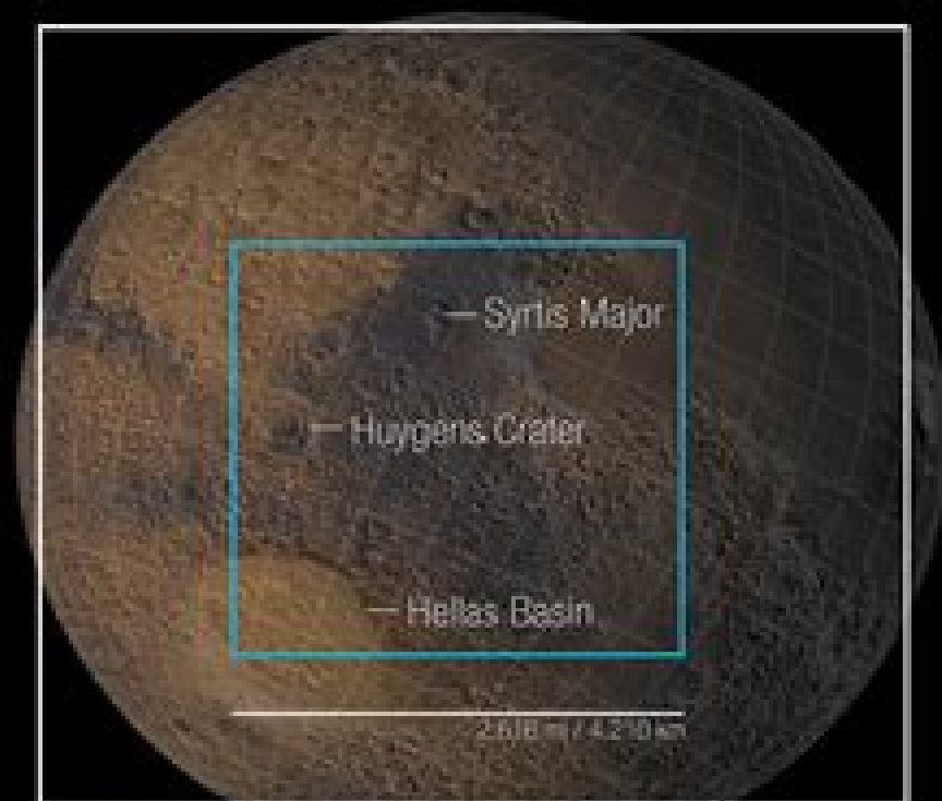
Simulated image with base maps from NASA and MOLA data
