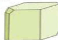
kyanite
