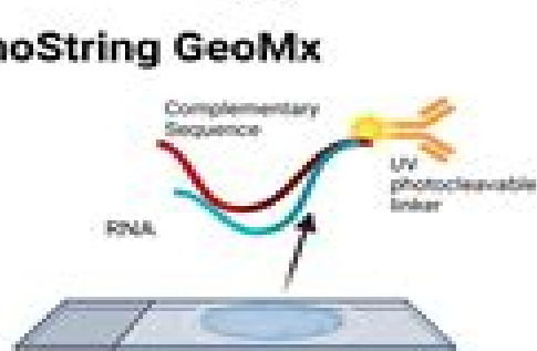
1. Staining/hybridization
