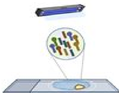
2. UV cleavage
