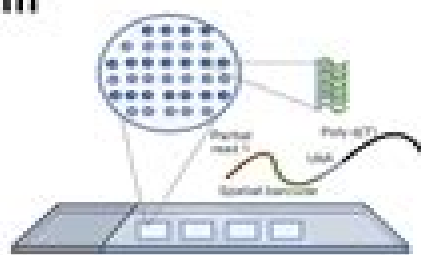
1. Sample preparation
