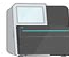
4. Sequencing
