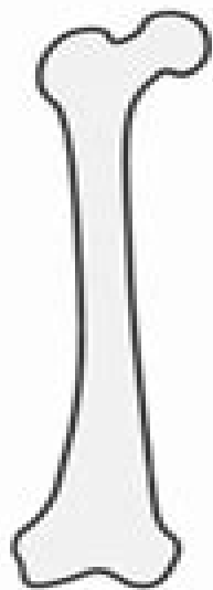
Normal
