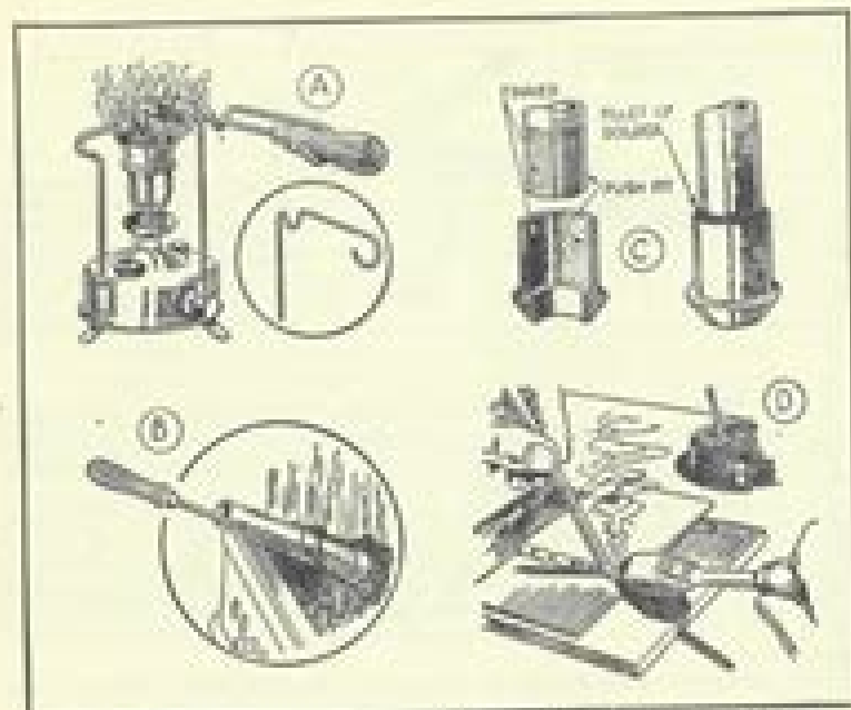
If a Primus stove is used for heating the soldering iron, it should be provided with a wire bracket (A); and a tube (B) in addition if a coal or coke fire is used, so as to keep the iron clean. (C) This is the way to fix a nipple to a pipe and (D) to join two sheets of metal.
