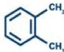
Ortho-xylene
