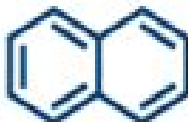
Napthalene
