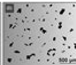
Lack of fusion (incomplete or partial melting)
