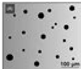
Gas/keyhole pores
