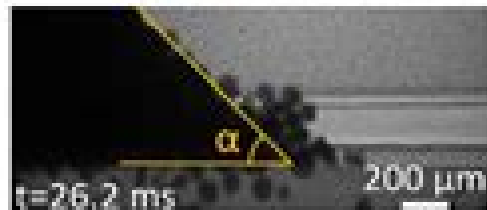
Powder spreading
