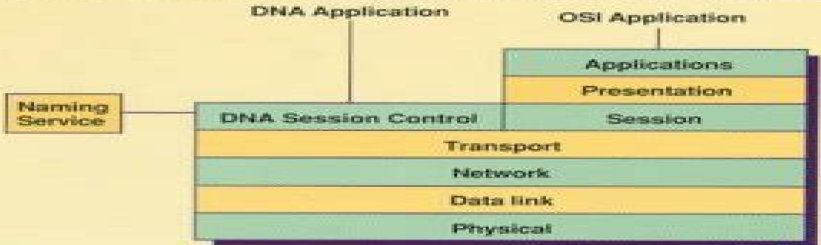
DECnet Phase V Architecture
