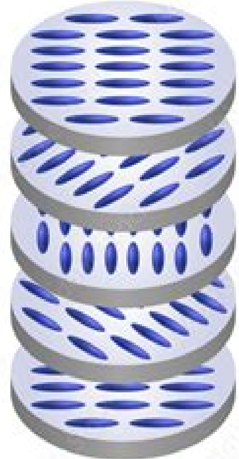
Cholesteric Phase
