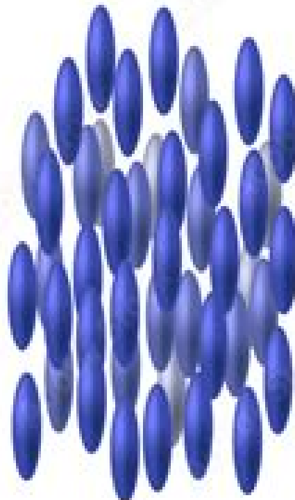
Nematic Phase
