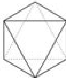
OCTAHEDRON
