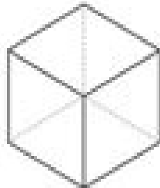
HEXAHEDRON
