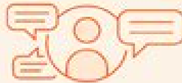
Answering questions
