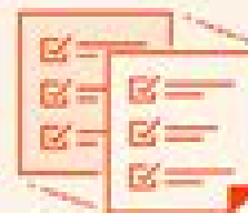
Machine translation
