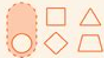
Text classification
