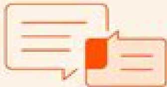
Language generation
