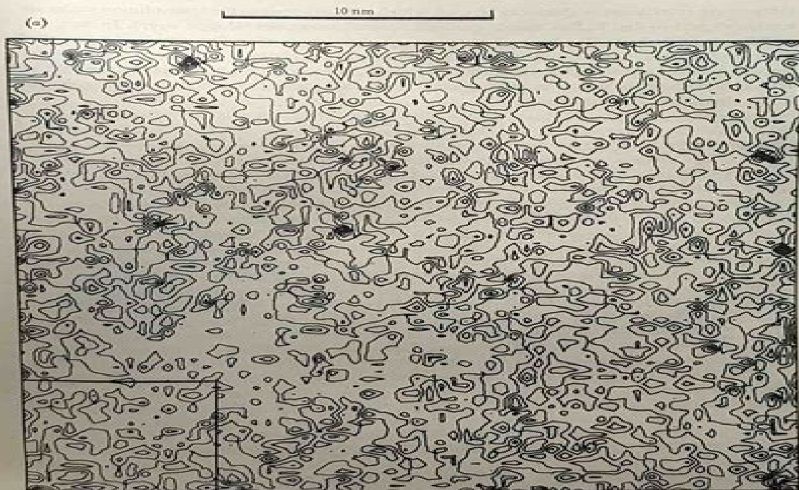
FIGURE 12. Difference image of an amorphous carbon foil, 10 to 20 nm thick. The two original micrographs were registered with the same electron optical parameters ( \lambda = 3.7 pm, C_s = 3.9 mm; z_s = 410 nm, \Delta f_s = 124 nm) at a magnification of 180 000 on photographic films. The difference image shows the change of the foil after an electron bombardment of 80 000 to 110 000 electrons per square nanometre in the microscope. The total pressure of the residual gases in the microscope (Elmiskop 1a) was about 10^{-4} Torr ( 13 \mu\text{N m}^{-2} ); the specimen was surrounded by a chamber cooled down to liquid nitrogen temperatures. In (a) the difference between two successive lines of equal intensity corresponds to a step \Delta S = 0.05 of the registered optical density; lines of positive and negative values are not distinguished. The resolution of the map is 0.45 nm, i.e. for mapping all Fourier coefficients with d^* = (1/d) > (1/0.45 \text{ nm}) were set to zero. In the lower corner on the left of figure 12a the region is marked which is shown in figure 12b in more detail: resolution 0.3 nm, difference between two successive lines of equal optical density \Delta S = 0.03 . High maxima are marked by the symbols A 0, A 1, ..., E 9, A 0 denoting the highest value and so on; low minima are marked by the symbols V 0, V 1, ..., Z 9, starting with the lowest value V 0. (c) finally shows the reconstructed difference image of (b) using the same contour level distances as in (b).
