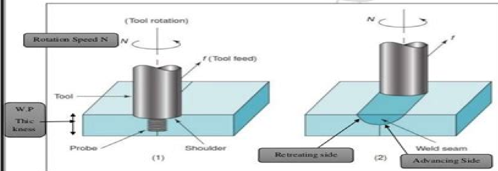
Figure 1. Friction stir welding (FSW): (1) rotating tool just prior to feeding into joint and (2) partially completed weld seam. N =tool rotation, f =tool feed.
