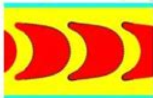
Capillary Flow of Red Blood Cells
