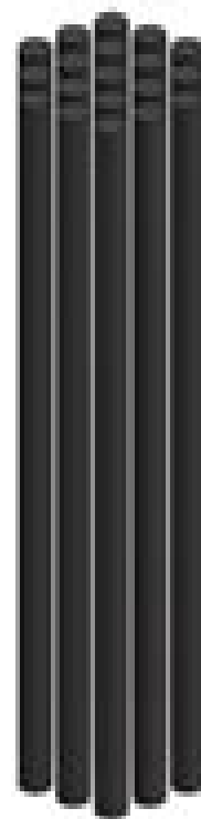
CARBON FIBERS
