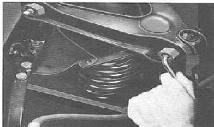
Fig. 1—Turning Pivot Pin to Set Caster and Camber
