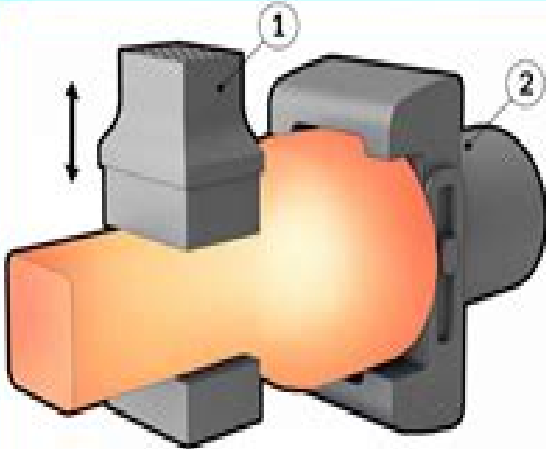
Open and Closed Die Forging Processes
