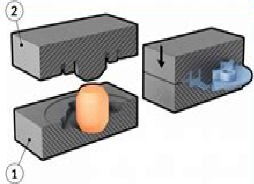
Open and Closed Die Forging Processes
